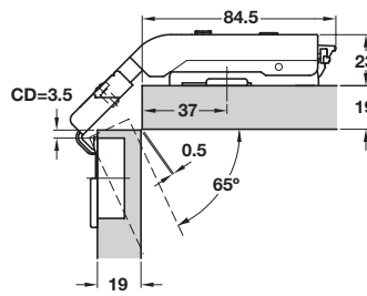
19 mm door thickness (factory setting) Mounting plate height 0 mm
