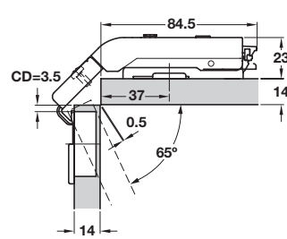
Mounting plate height 0 mm
