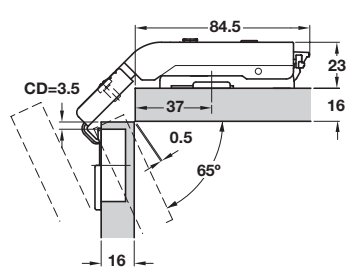
Mounting plate height 0 mm
