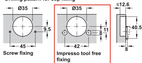
Drilling pattern for cup fixing
