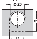
Drilling pattern for cup fixing
