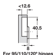
For 95°/110°/120° hinges
