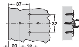
For Hospa screws
