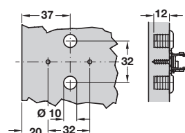
With dowel fixing
