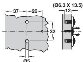
With pre-mounted Euro screws
