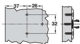
For Hospa screws
