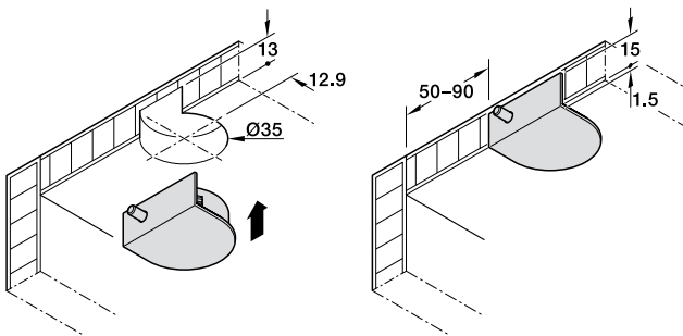
For recess mounting
