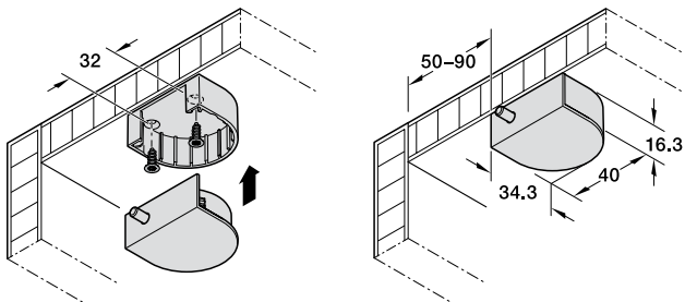
For surface mounting
