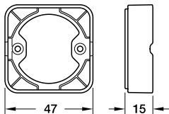
Housing for undermounted light
