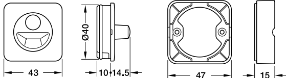
Housing for undermounted light
