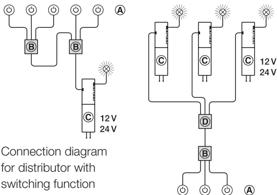
Connection diagram for distributor with switching function
