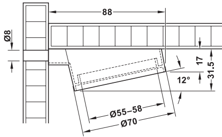
Surface mounting, angled
