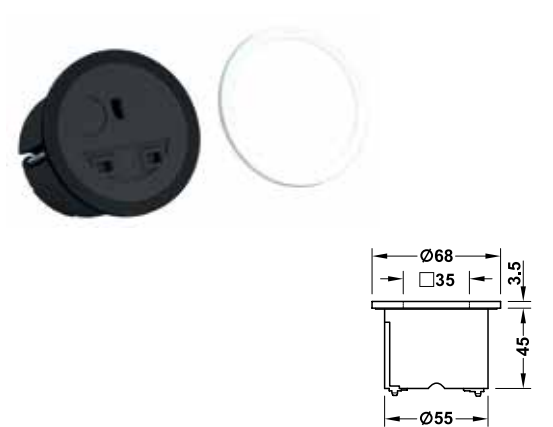
BACHMANN PIX socket
