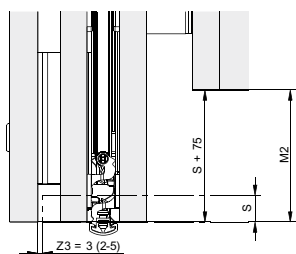
Retracted door leaf flush with the outside
