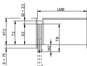
Retracted door leaf protruding
