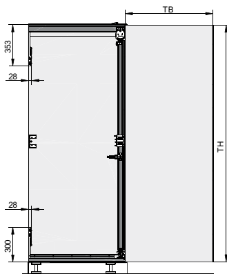
Retracted door leaf flush with the outside
