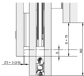
Retracted door leaf protruding
