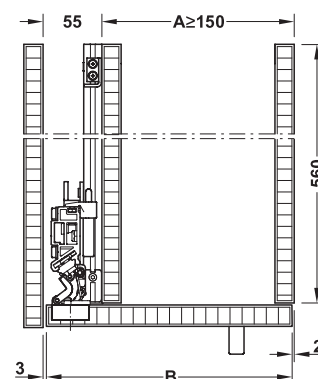
Section top view closed (parking pocket for 1 door)
