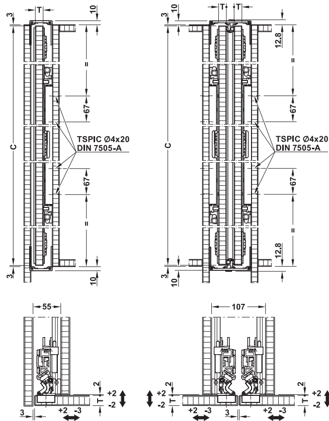
Parking pocket for 1 door
