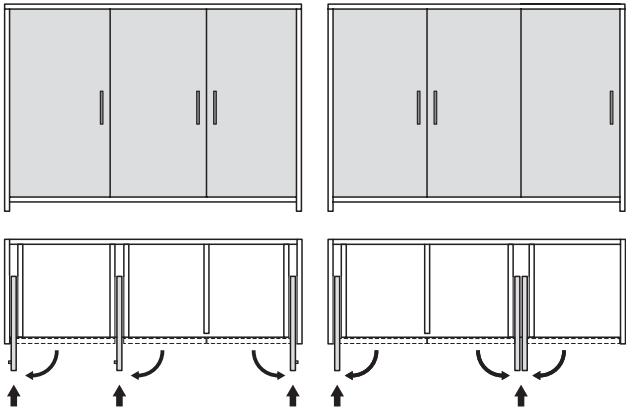
Parking pocket for 1 door
