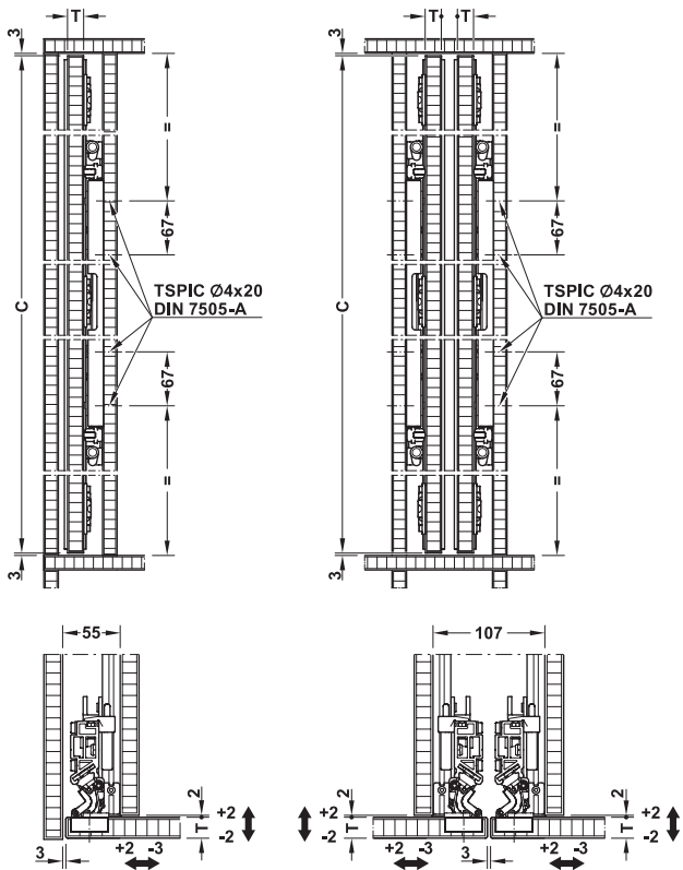
Parking pocket for 1 door
