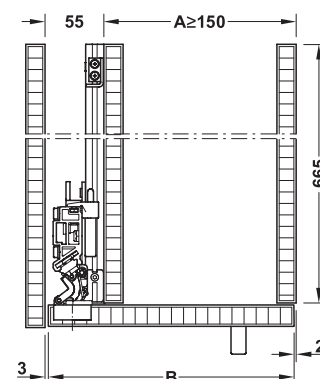
Section top view closed (parking pocket for 1 door)
