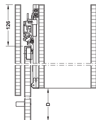
Section top view open (parking pocket for 1 door)
