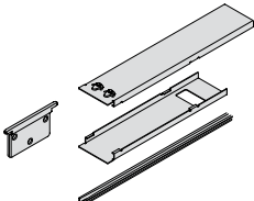
Parking pocket for 2 door leaf version
