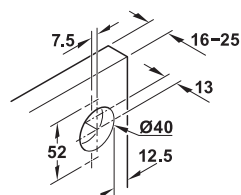
Drilling pattern for cup fixing
