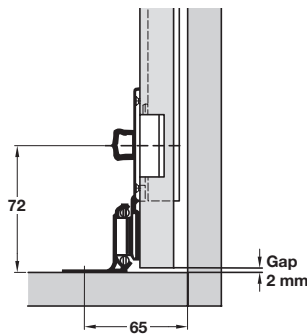
Mounting diagram for doors opening normally (vertical use)
