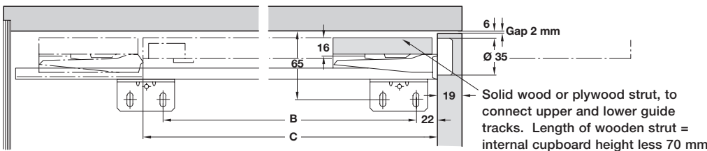
Mounting diagram for doors or flaps opening upwards (horizontal use)
