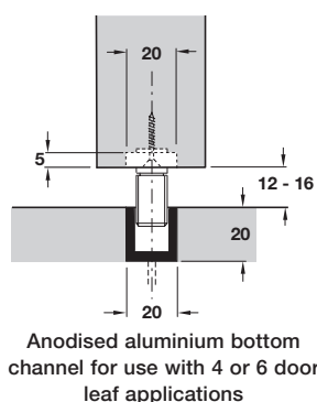
Section through typical door/pivot
