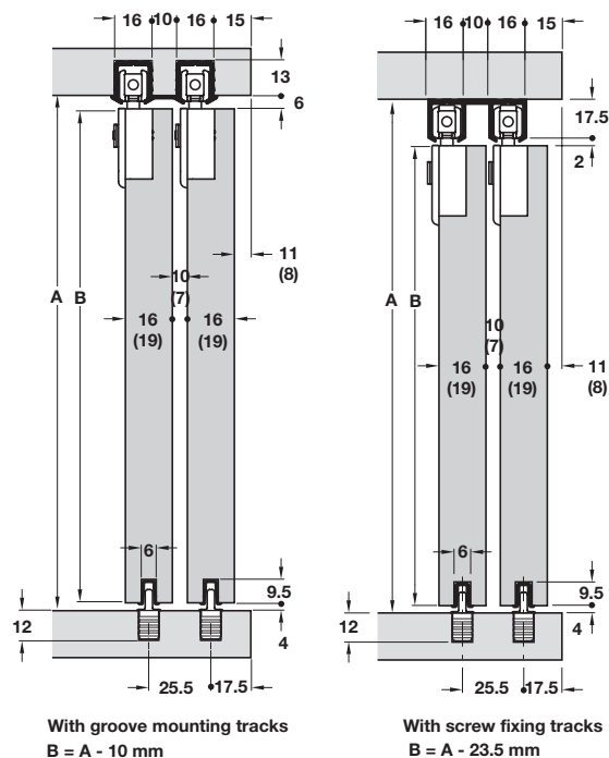
Installation dimensions
