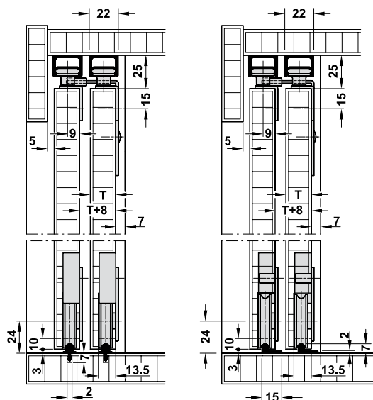
Guide track groove mounted
