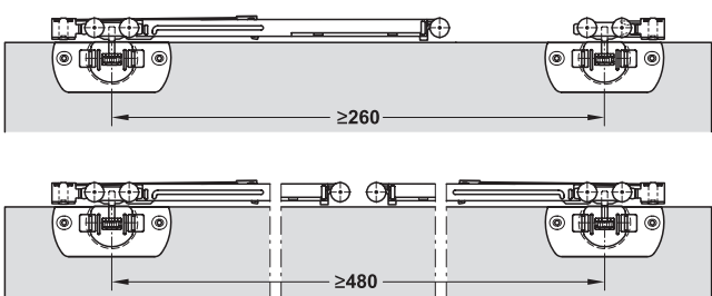
Installation of (optional) soft close
