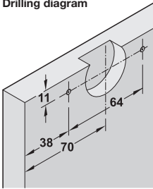
Drilling diagram
