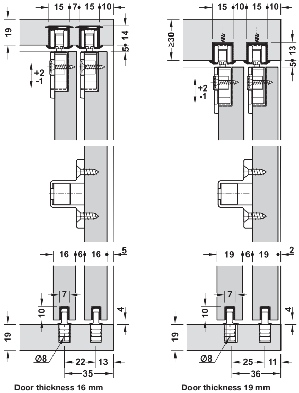
Door thickness 16 mm
