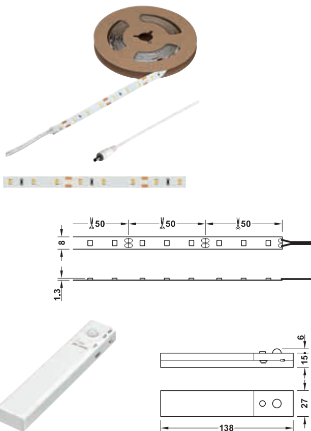
Supply unit with motion sensor, for battery operation
