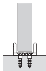
Standard bottom guiding
