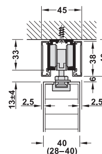
Ceiling installation with clip panel
