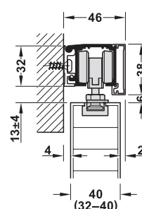
Wall mounting with clip panel
