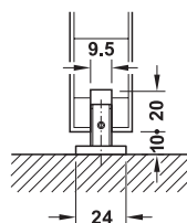
Wall mounting with clip panel
