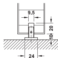
Wall mounting with clip panel
