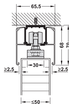
Ceiling installation with clip panel
