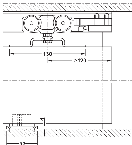
Section trolley hanger and guide
