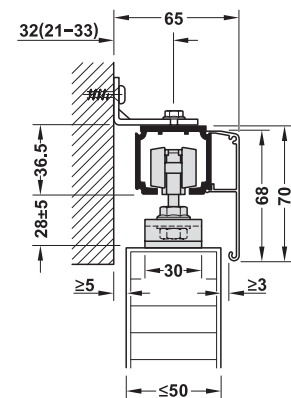
Wall mounting with clip panel
