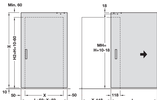
Cut-out dimensions
