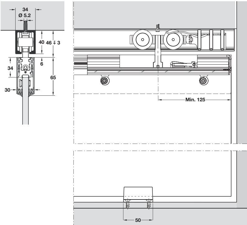
Glass cut-out detail Only toughened safety glass (ESG) should be used
