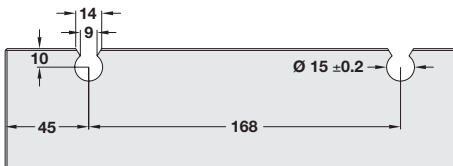
Glass cut-out detail Only toughened safety glass (ESG) should be used
