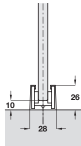
Bottom guiding with guide, without channel; page 2.45
