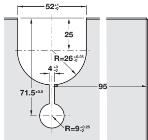
Glass cut-out detail
