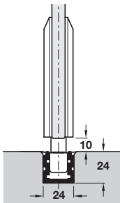
Bottom guiding with patch assembly; page 2.47
