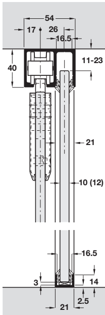
HAWA-Junior 80/GP with fixed glass
