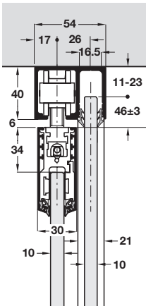
HAWA-Junior 80/GL with fixed glass
