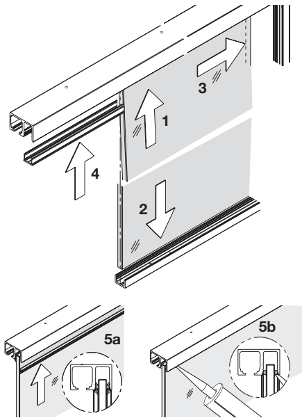
HAWA-Junior 80/GL with fixed glass
