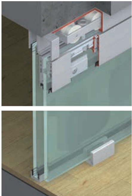
HAWA-Junior 80/GP with fixed glass
