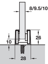
Bottom guiding with floor guide H
