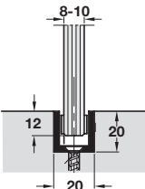
Bottom guiding with sliders F and channel G
