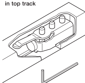
The retaining force can be adjusted with an allen key
