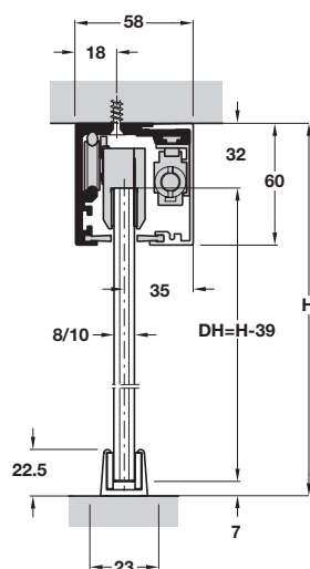
Ceiling installation and wall mounting
