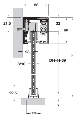
H = Total height DH = Door height
