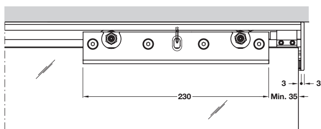
Section trolley hanger 120 kg
