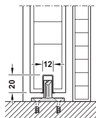
With guide track
