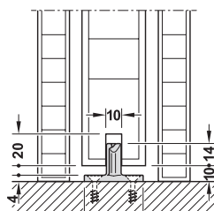
Without guide track
