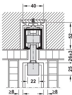
Integrated ceiling installation with long hanger bolt (+20 mm)
