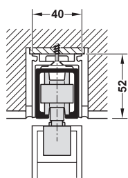
Integrated ceiling installation
