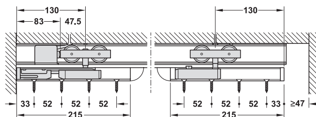
Section trolley hanger
