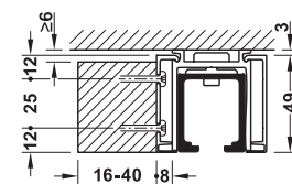
Panel with material thickness of up to 40 mm can be installed
