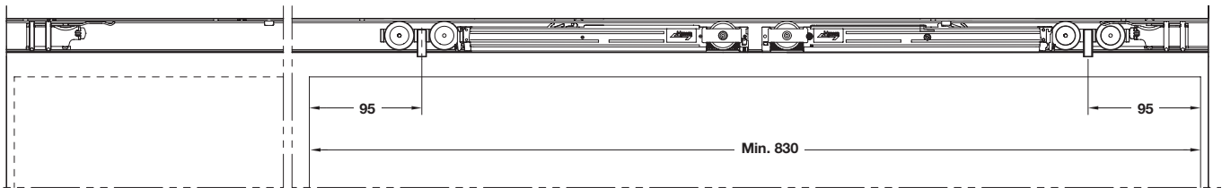
Two-sided damping
