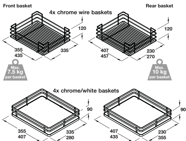
Cabinet mechanism
