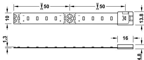
833.76.241 - LED 3015 flexible strip light
