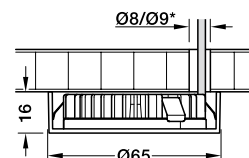
4x 833.72.126, recess mounting bezel
