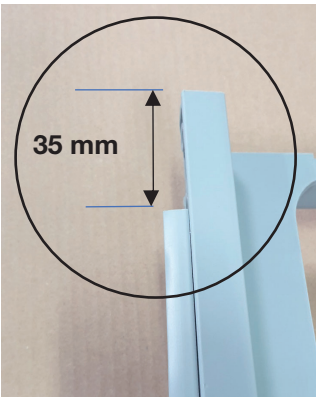
Moores special version uses a shorter rubber side strip - 35 mm shorter at the back
