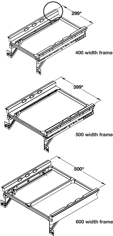
Moores special version uses a shorter rubber side strip - 35 mm shorter at the back
