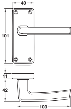
901.78.371 Backplates for latch
