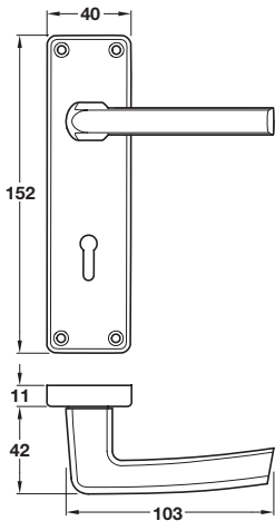
901.78.372 Backplates for lever lock
