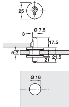
Glass aperture diagram
