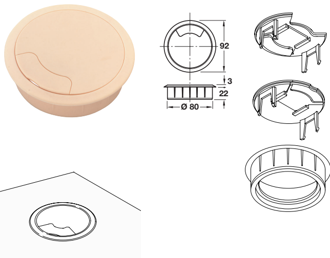
A Cable outlet, Ø 80 mm
