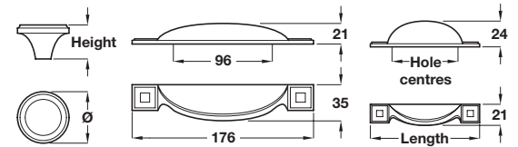
Knob, round
