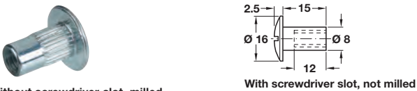
Without screwdriver slot, milled
