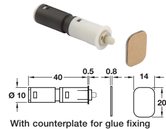
With counterplate for glue fixing
