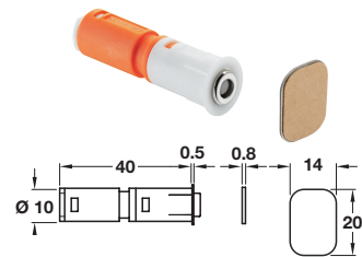
Additional catch (without eject pin) and counterplate, for door fronts over 1200, glue fixing
