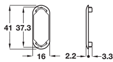
Oval cover cap for 12 x 36 mm hole
