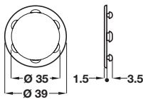
Round cover cap for Ø 35 mm hole
