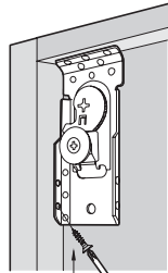
Fixing
