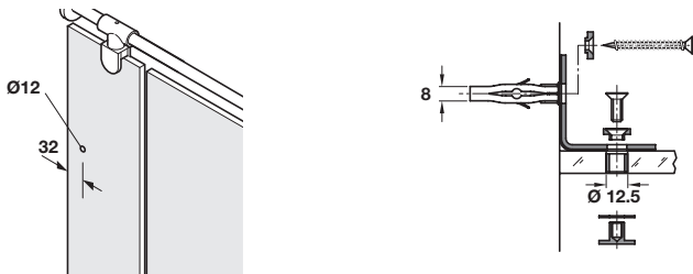
Glass to wall
