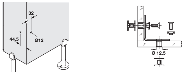
L junction glass to glass
