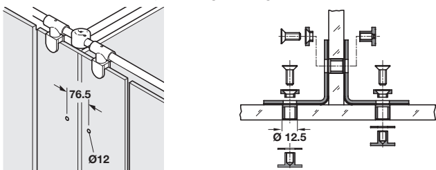
T junction glass to glass
